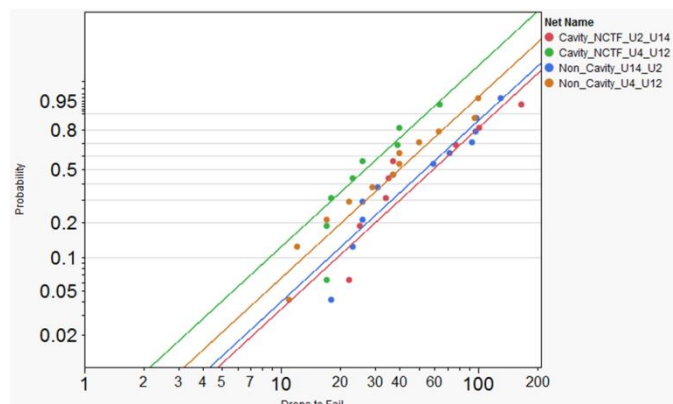
Figure 14. Cavity and Non-cavity solder joint joint reliability, NCTF locations
