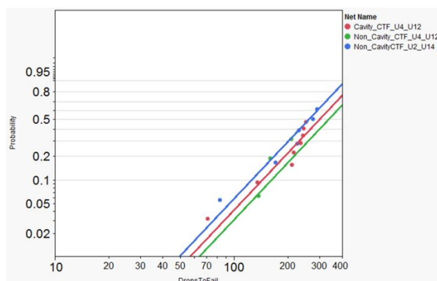
Figure 15. Cavity and Non-cavity CTF solder reliability
