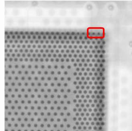
X-ray - Layer 4 Insufficient Paste
