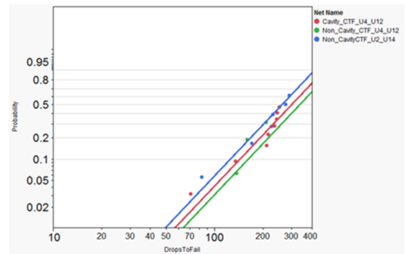
Figure 15. Cavity and Non-cavity CTF solder joint reliability. Note: No CTF failures observed at the U2 and U14 cavity locations.
