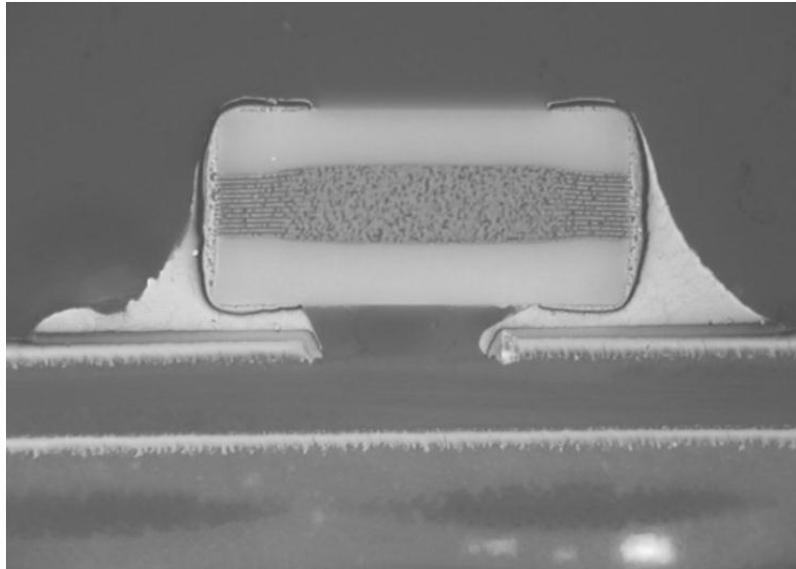
01005 Reflow in Air
