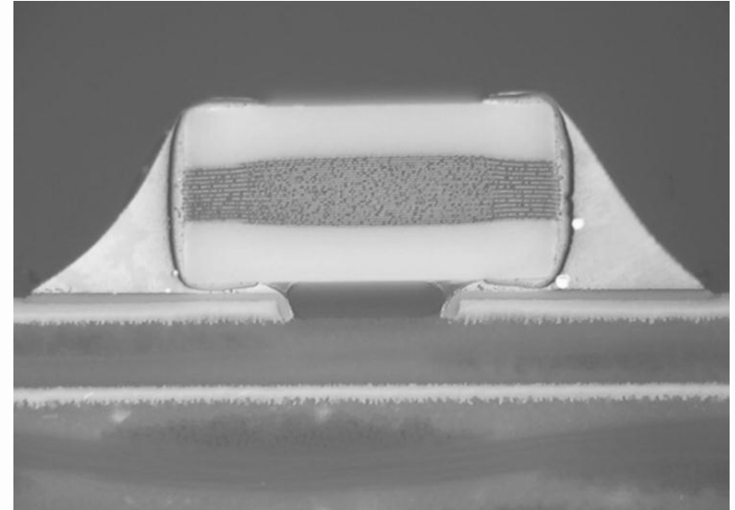
01005 Reflow in Nitrogen
