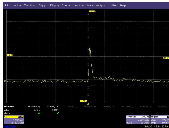
Figure 14: Shape of Discharge Current Waveform emitted by Charge Generation Tool.
