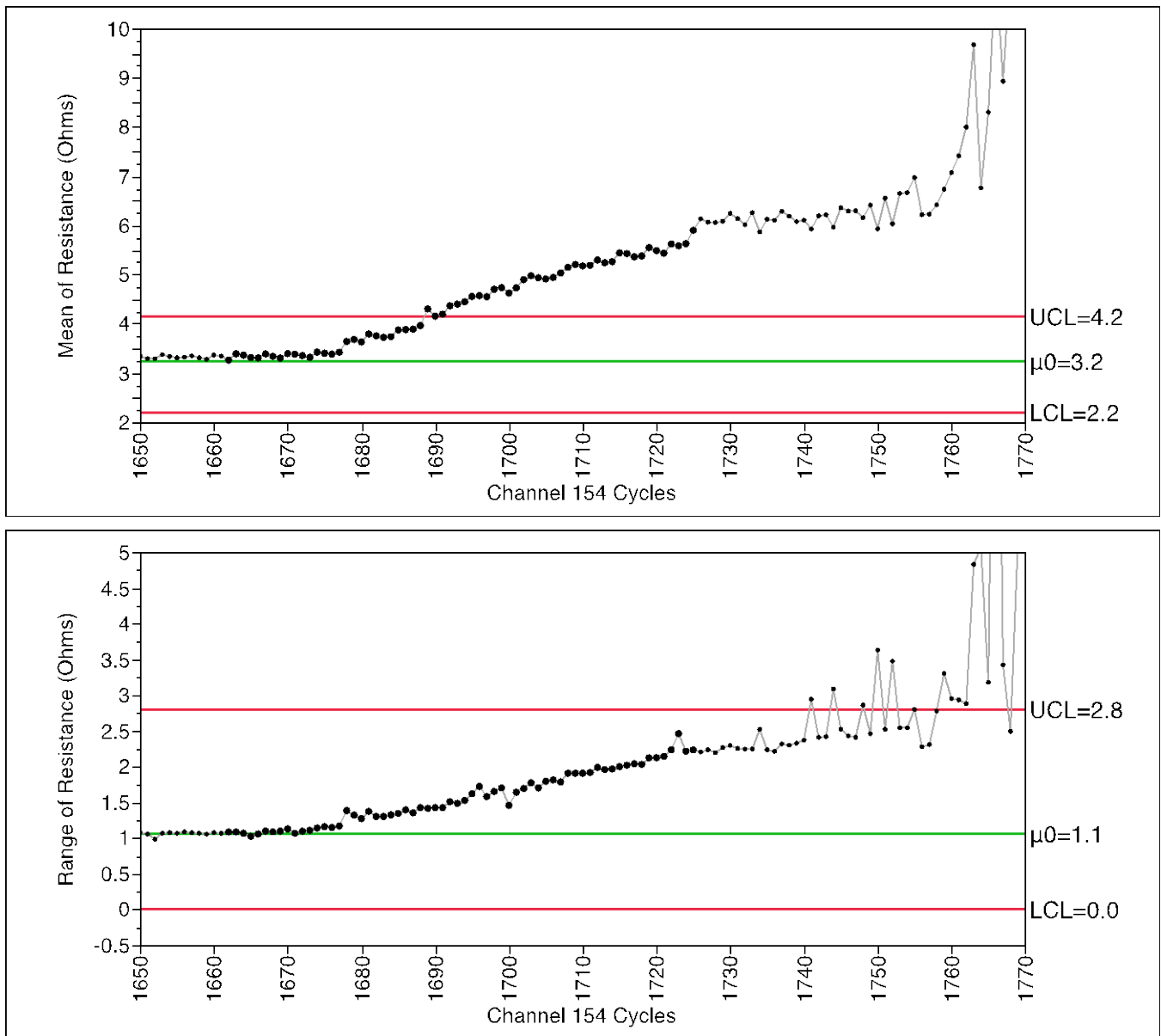
Figure 8. Resistance behavior of Channel 154, (top) mean of resistance from Cycle 1650 to Cycle 1770, (bottom) range of resistance from Cycle 1650 to Cycle 1770.
