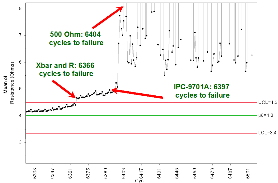
Figure 4. Comparison of cycles-to-failure between the control-chart based method, IPC 9701A, and the 500 \Omega resistance threshold for one daisy-chain.
