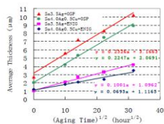
Figure 14 – Bonding Strength Decreasing by IMC Thickness 4
