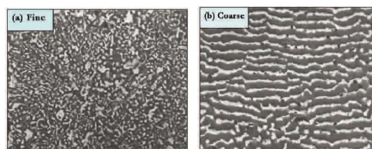
Figure 29 –Cooling Rate Effect on Grain Size 9
