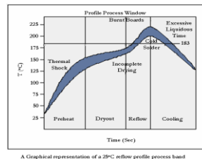
Figure 27 – Reflow Profile
