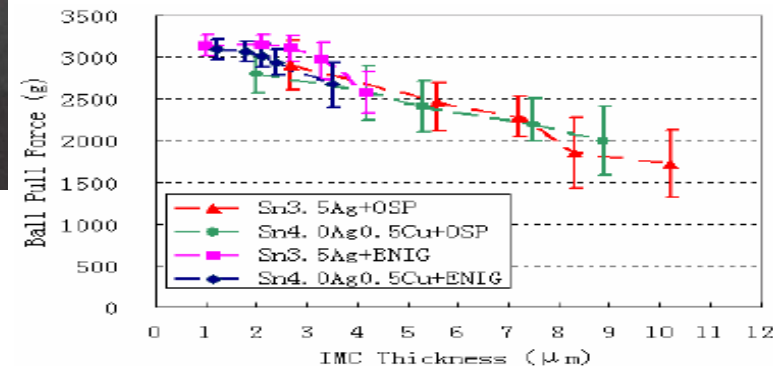
Figure 20. Effect of IMC thickness on the ball pull strength (Pull speed: 5000 \mu\text{m/s} )
