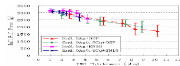
Figure 20 – Effect of IMC thickness on the ball pull strength (Pull speed: 5000 um/s)
