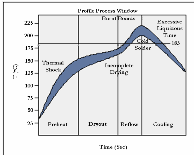
A Graphical representation of a 25°C reflow profile process band
