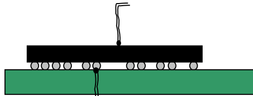
Figure 30 - Thermocouple Location
