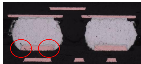
Figure 4 – Cross Section of NSMD
