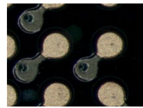
Figure 6 – Via out of Pad
