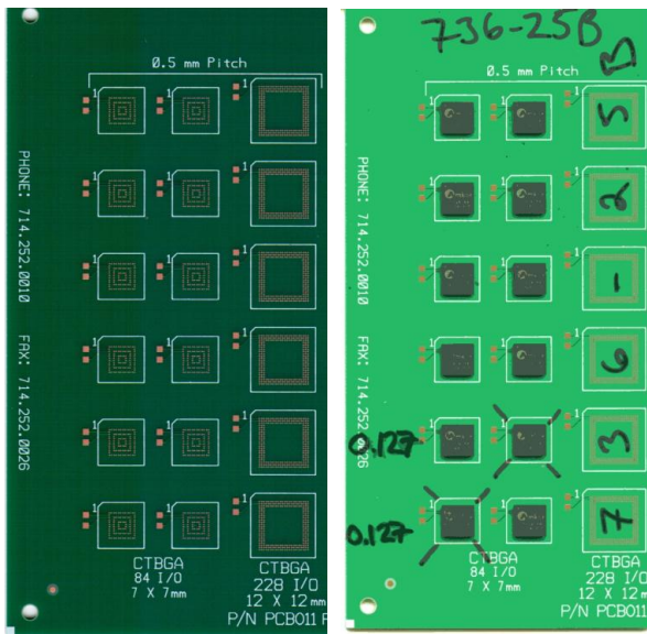
Figure 6 Test board used in demonstration of Epoxy Flux A before and after BGA assembly.
