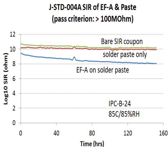
Figure 19 SIR of epoxy flux A on solder paste per J-STD-004A
