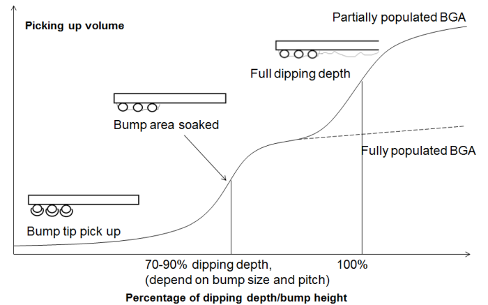
Figure 7 Relation between the flux pick-up volume, the ratio of dipping depth/bump height, and the bump pattern of the BGA.
