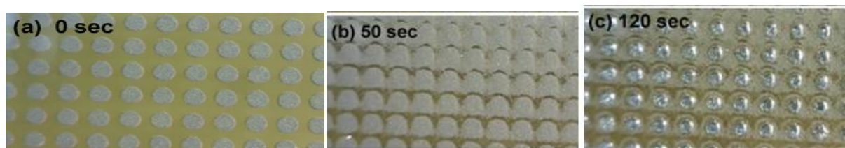
Figure 1 Reflow progress of printed solder paste immersed in epoxy flux and covered with a glass slide on a 250°C hot plate.
