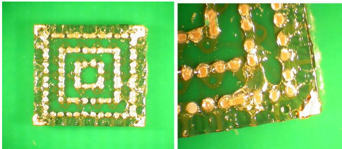
Figure 11 Bottom view of a BGA assembled with epoxy flux A after being pried off.
