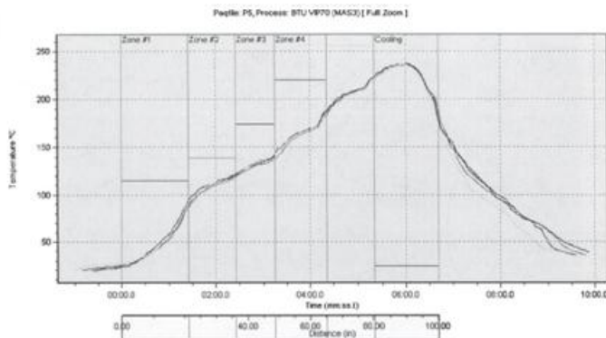
Figure 8 Reflow profile used in this study
