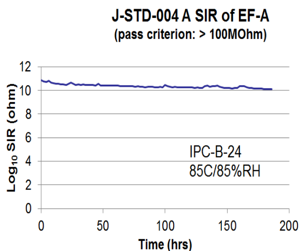
Figure 18 SIR of epoxy flux A per J-STD-004A
