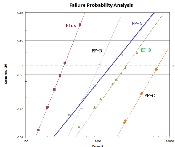
Figure 17 Weibull analysis on drop test results of assembled CTBGA84
