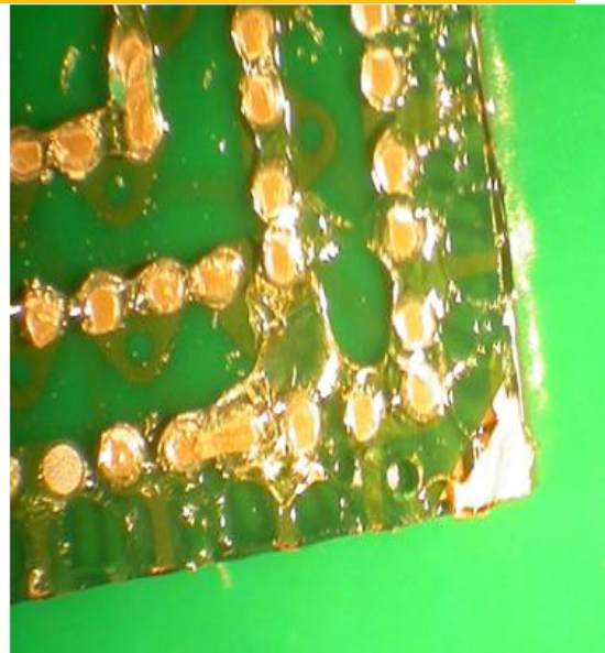
BGA side
