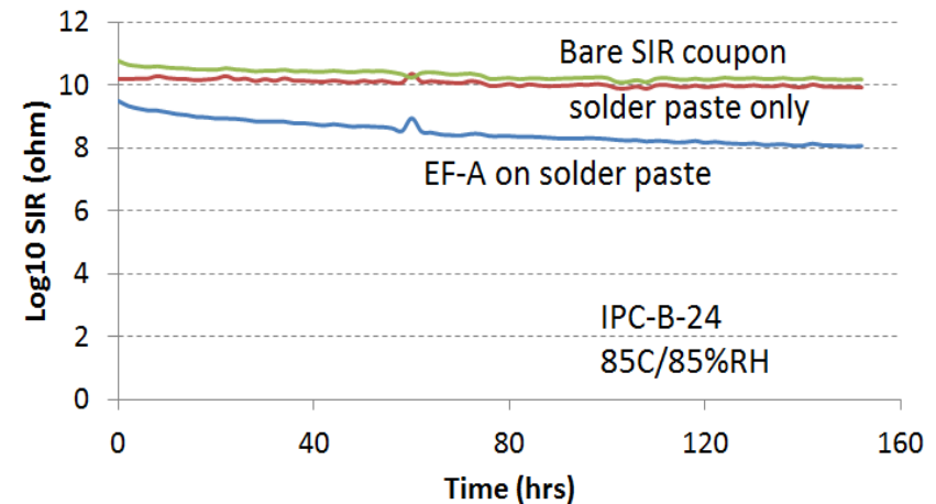
J-STD-004A SIR of EF-A & Paste (pass criterion: > 100M \Omega m)
