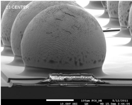
Figure 21 WLCSP ball mounting with epoxy flux E.
