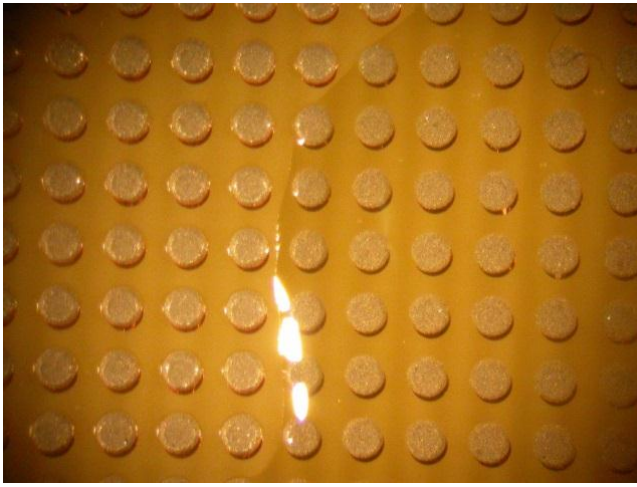
Figure 2 Demonstration with half of the paste dots covered with epoxy flux A (right side) without the paste oozing out.
