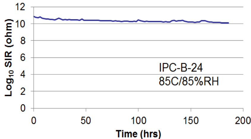
J-STD-004 A SIR of EF-A (pass criterion: > 100M \Omega m)
