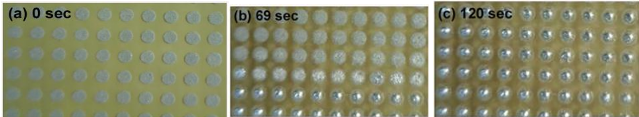
Figure 4 Reflow progress of printed solder paste immersed in epoxy flux A and covered with a glass slide on a 250°C hot plate.
