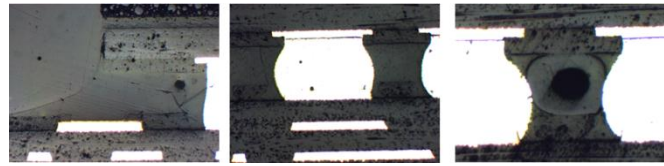
Figure 10 Cross-sections of BGA joints assembled with epoxy flux A.
