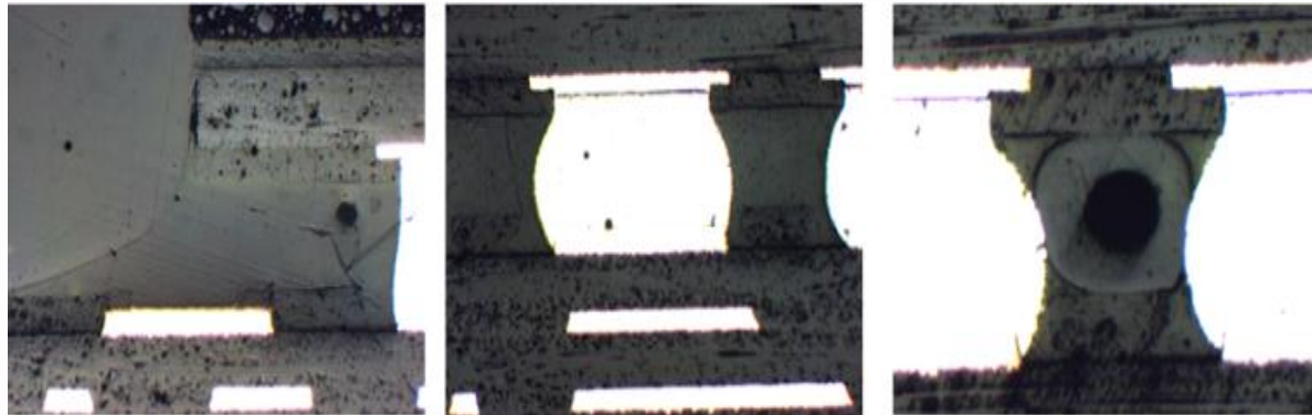
Cross section of a component installed with epoxy flux
