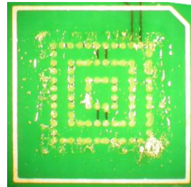
Figure 12 Top view of the PCB after the BGA assembled with epoxy flux A was pried off.
