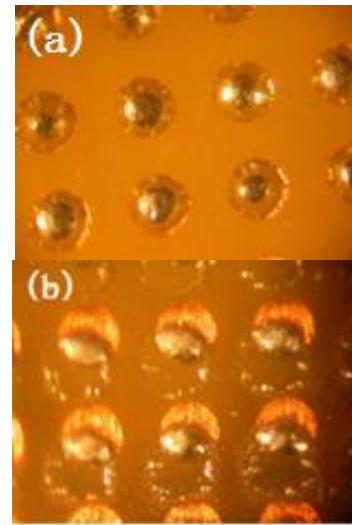
Figure 3 Photo of the solder paste covered with epoxy flux A (a) and an epoxy flux without designed-in compatibility (b) after being reflowed on hot plate.
