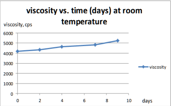
Figure 20 Viscosity stability of epoxy flux A at room temperature.
