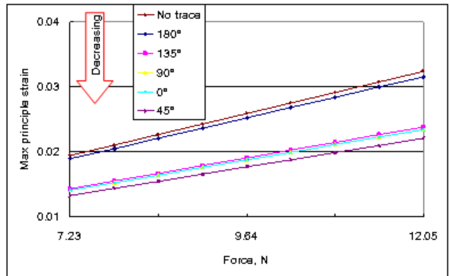
Figure 12. Max principle strain VS. pulling force with different angle of copper trace
