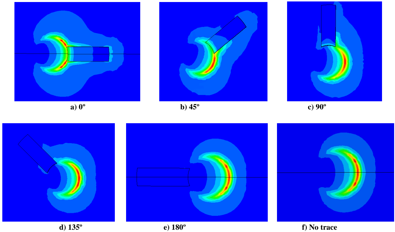
Figure 11. Contour of principle strain of PCB with different angle of copper trace
