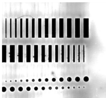
Figure 23 - Best Stencil for Bottom Side Paste Smear
