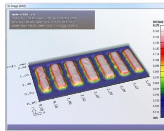
Good 2 Stencil 4 10th print (Nano-Coat A) 150 \mu Aperture
