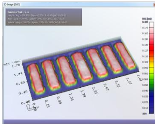
Good 2 Stencil 1 10th print (Nano-Coat A) 150 \mu Aperture
