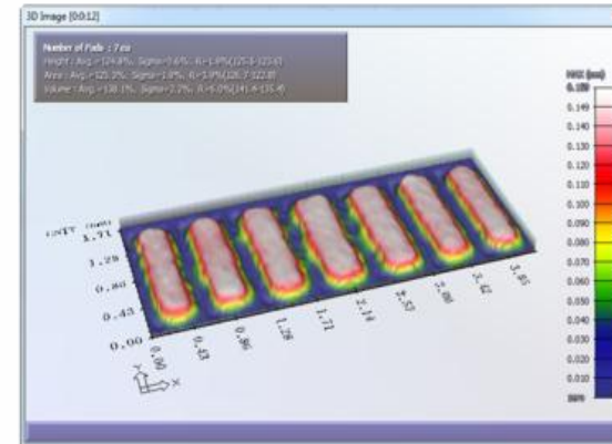
Good 2 Stencil 4 10th print (Nano-Coat A) 150 \mu Aperture
