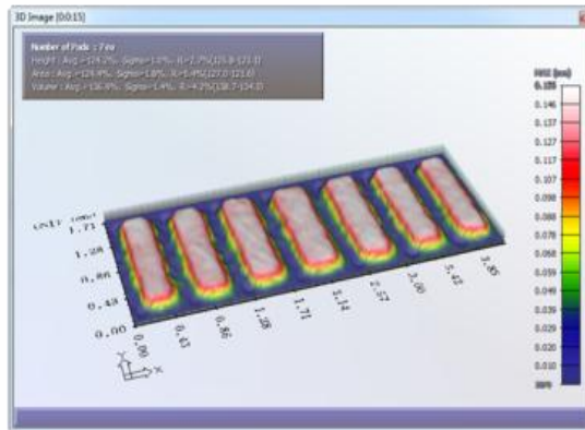
Good 2 Stencil 1 10th print (Nano-Coat A) 150 \mu Aperture
