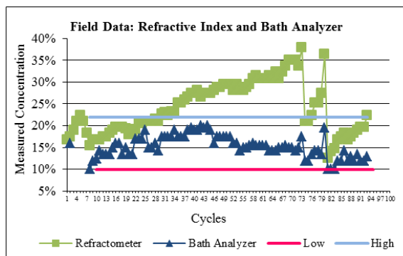
Figure 4. Field Data: Refractive Index and Bath Analyzer
