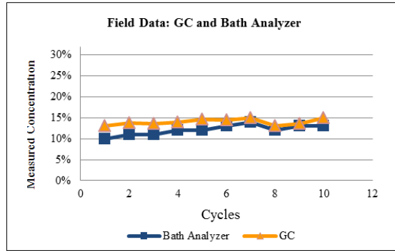
Figure 3. Field Data: GC and Bath Analyzer
