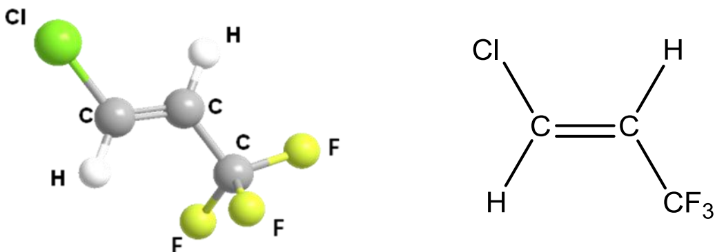
Fig 1 – Chemical Structure of Solvent 1233zd(E)
