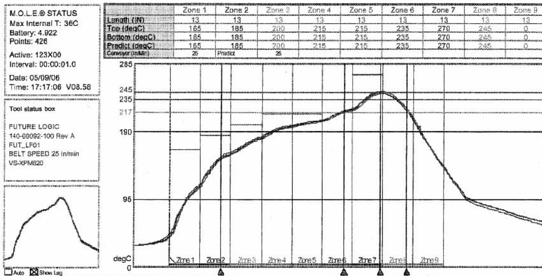
Figure 3 - Lead Free SAC305 water washable paste thermal profile
