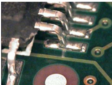
Figure 8 - Various SMD parts soldered well with SAC305; all met IPC-610 Class 1, 2, 3
