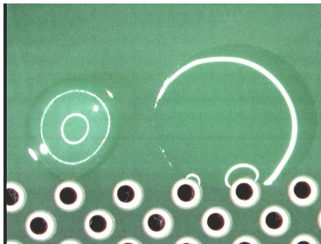
Figure 6. A drop of DI water and a drop of water-based flux on PWB solder mask. The surface tension of the water-based flux has been lowered by surfactants.
