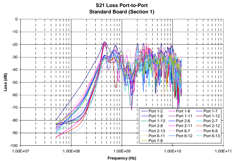
Figure 5 – S21 of Typical Board (Courtesy of IBM)
