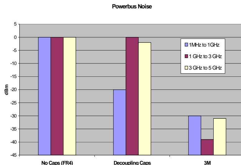
Figure 8 – Power Bus Noise (Courtesy of University of Missouri at Rolla)
