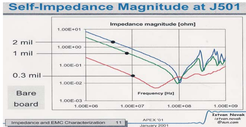
Figure 1 – Self-Impedance vs. Frequency (Courtesy of Sun Microsystems)
