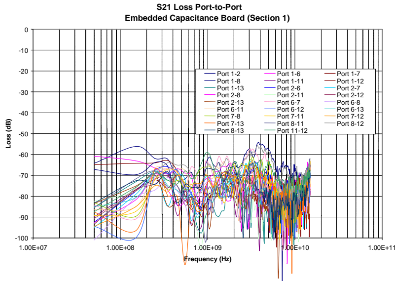
Figure 6 – S21 for Embedded Capacitance Board (Courtesy of IBM)
