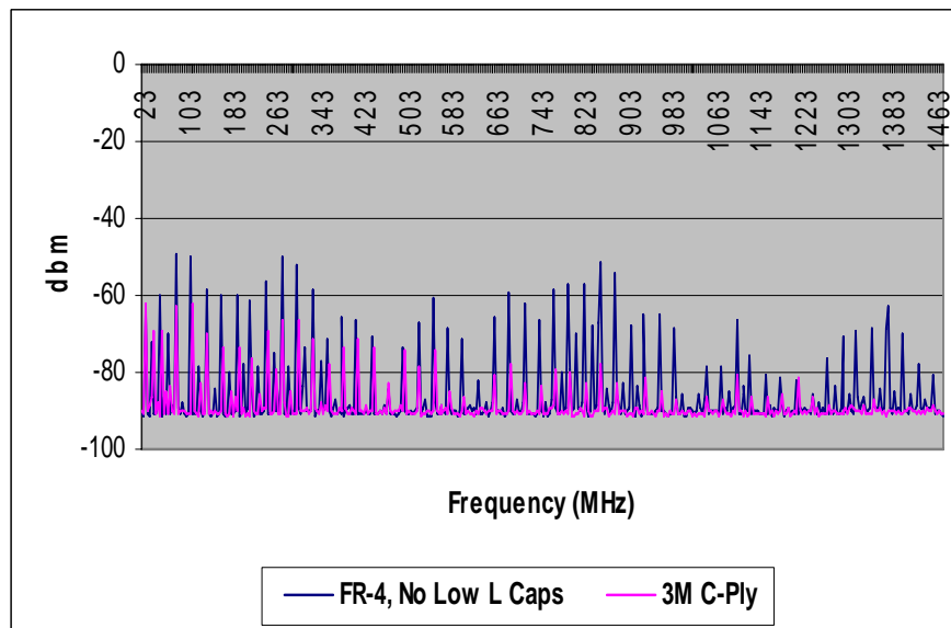
Figure 7 – Power Bus Noise vs. Frequency (Courtesy of H.P.)
