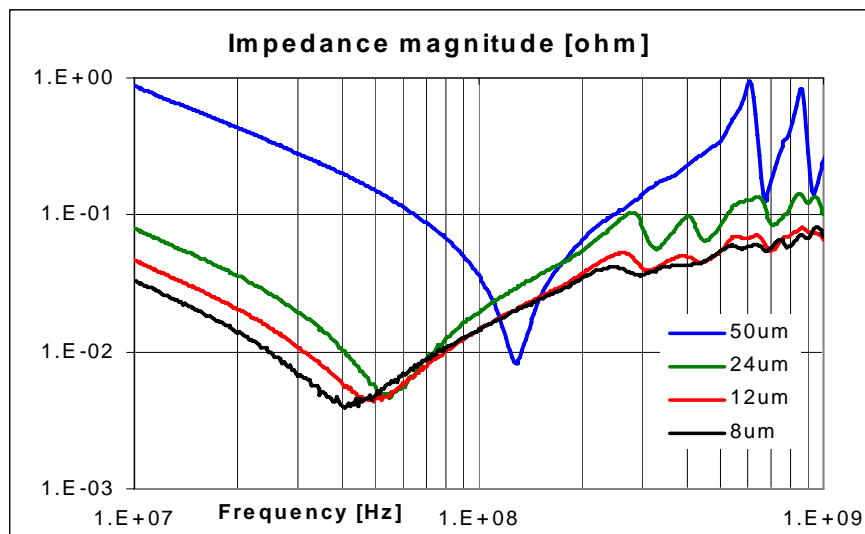
Figure 2 – Impedance vs. Frequency (Courtesy of Sun Microsystems)
