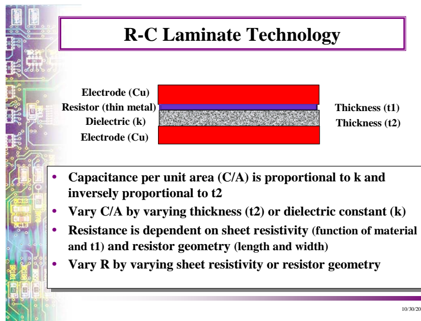
Figure 11 – R-C Laminate Technology
