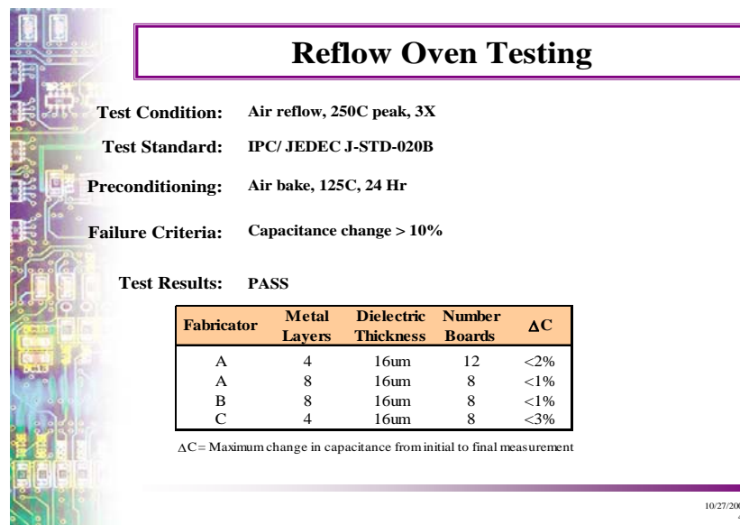
Figure 10 – Lead Free Reflow Simulation
