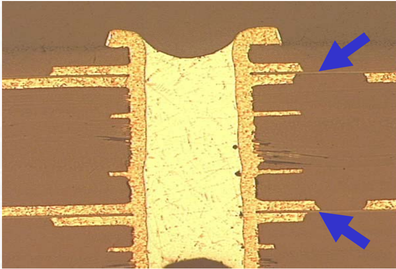
Two 3M C-Ply cores separated by an FR406 core.
