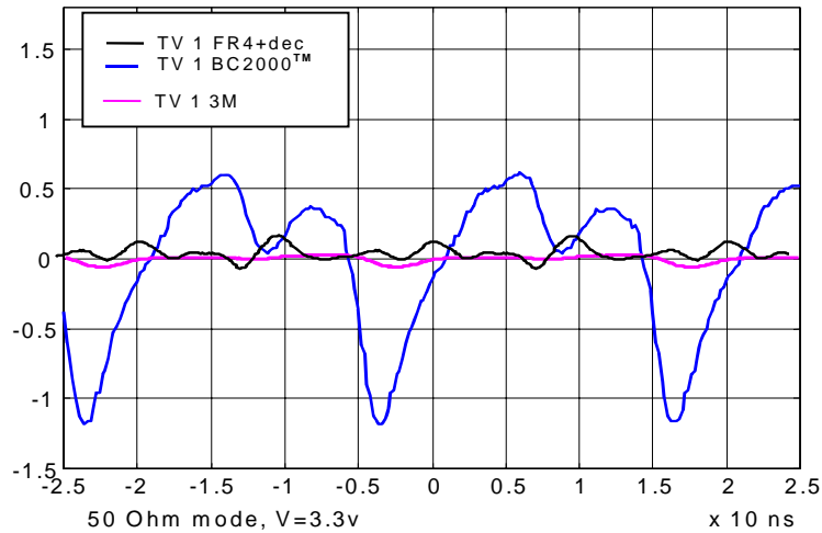
Figure 9 – Power Plane Voltage Fluctuation (Courtesy of University of Missouri at Rolla)
