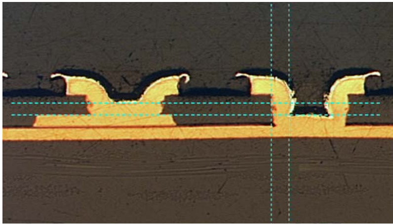
Figure 10 – Microvias in Test Board (Courtesy of Merix)
