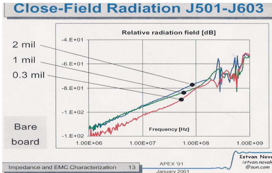
Figure 3 – EMI vs. Frequency (Courtesy of Sun Microsystems)
