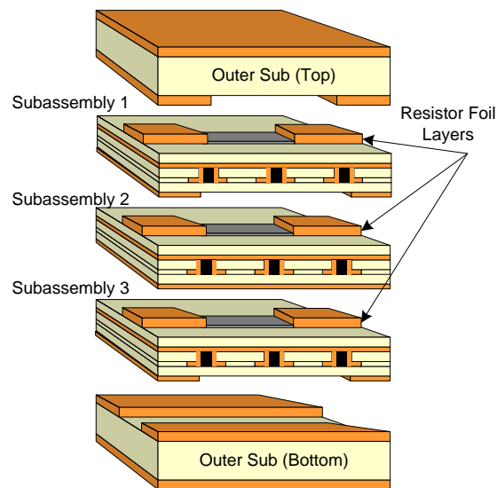
Figure 1 - Stack up of multilayer PCB with subassemblies and multiple embedded resistor layers.
