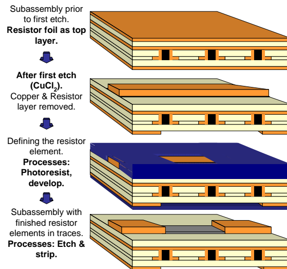
Figure 2 - Processes for Defining Resistor Elements
