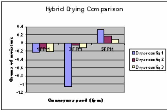
Figure 8 - Hybrid drying comparison for test board 3
