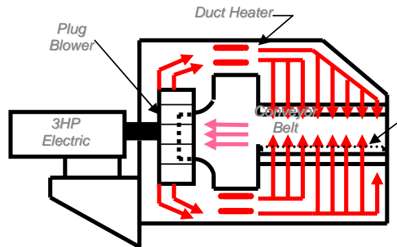
Figure 2 - High temperature convection heating zones
