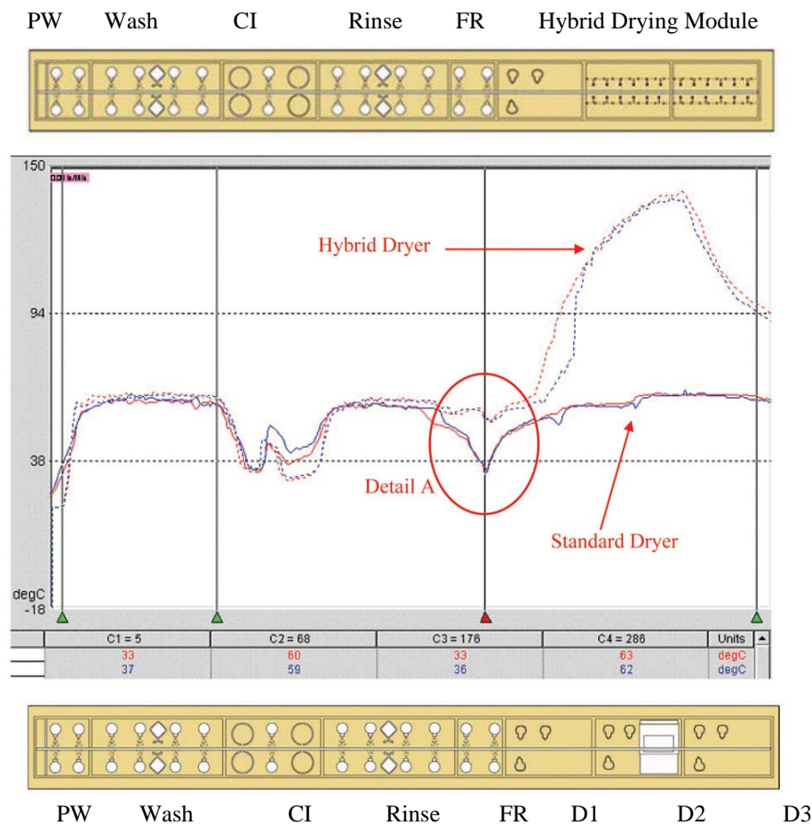
Figure 1 - In-line cleaning thermal profile
