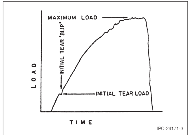
Figure 3 Load-time chart for high extensible base dielectric films
