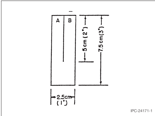
Figure 1 Single-tear specimens
