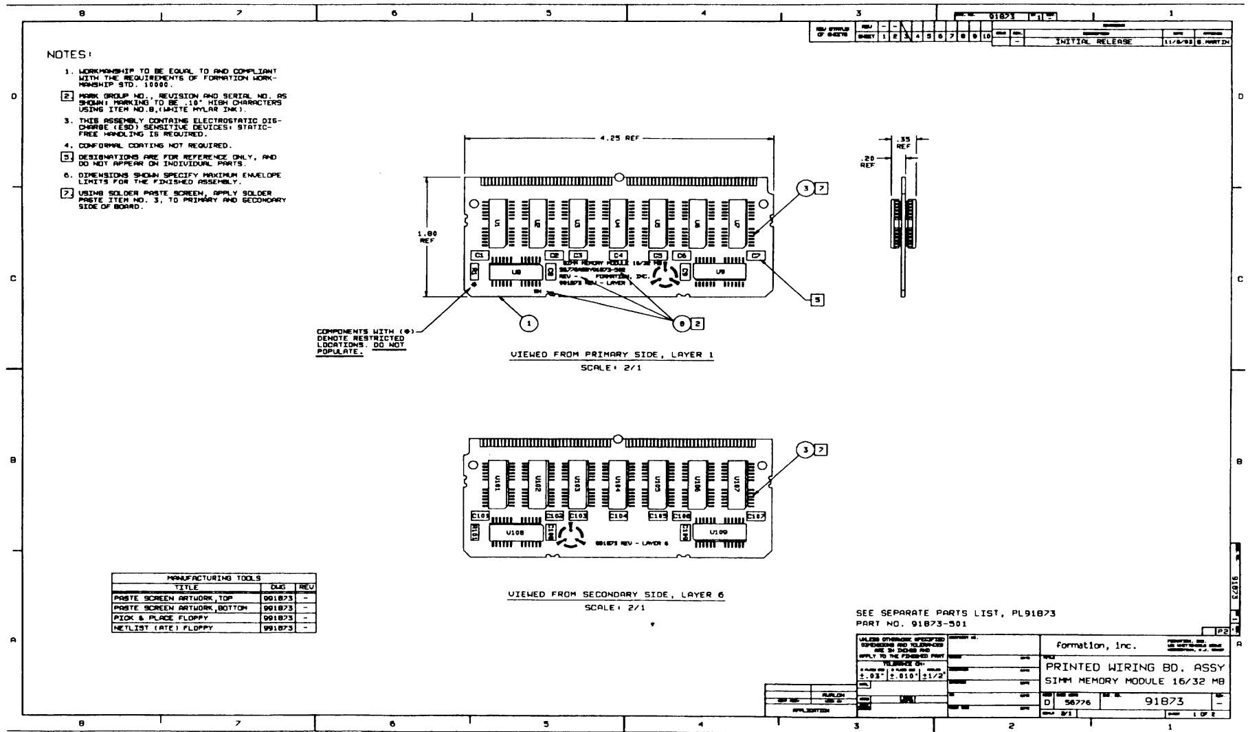
Figure 6-2 Assembly Drawing
