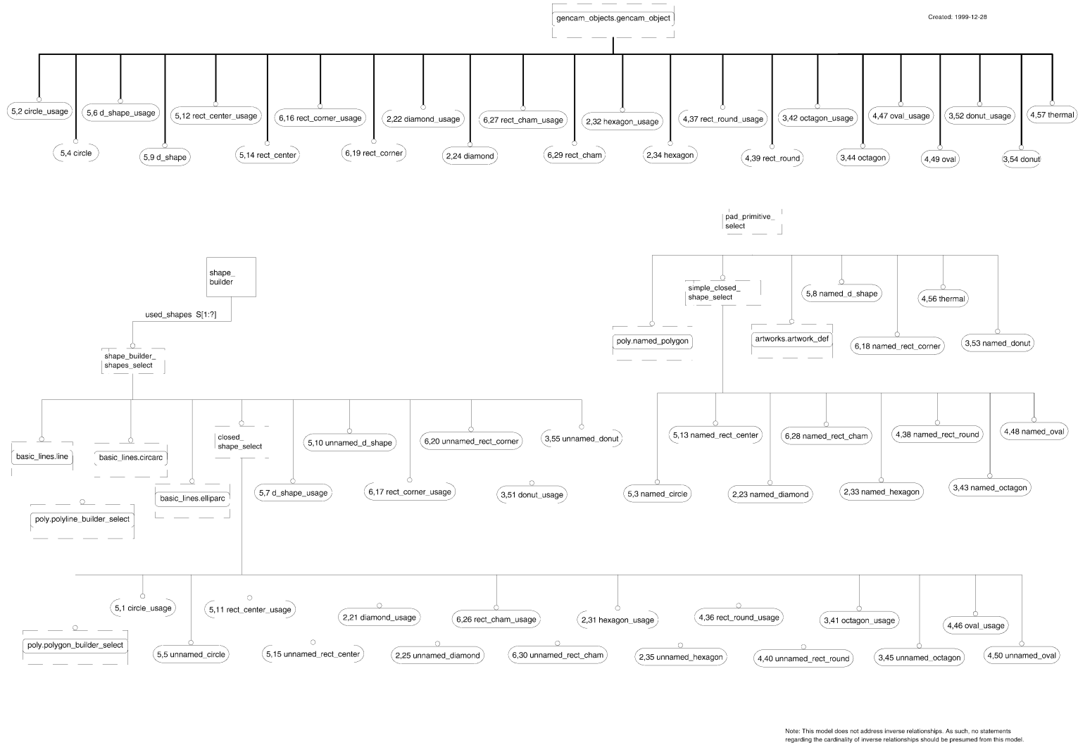
Figure 5-4 EXPRESS-G for PRIMITIVES
