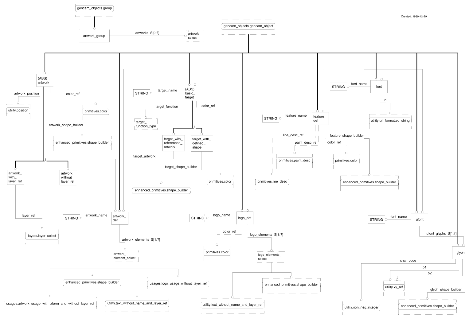
Figure 5-12 EXPRESS-G for ARTWORKS
