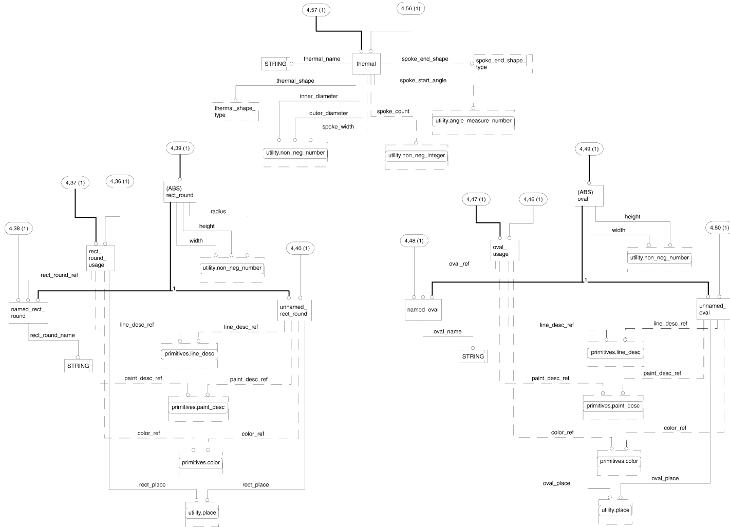
Figure 5-9 EXPRESS-G for Oval/Rectangle/Thermal Usage
