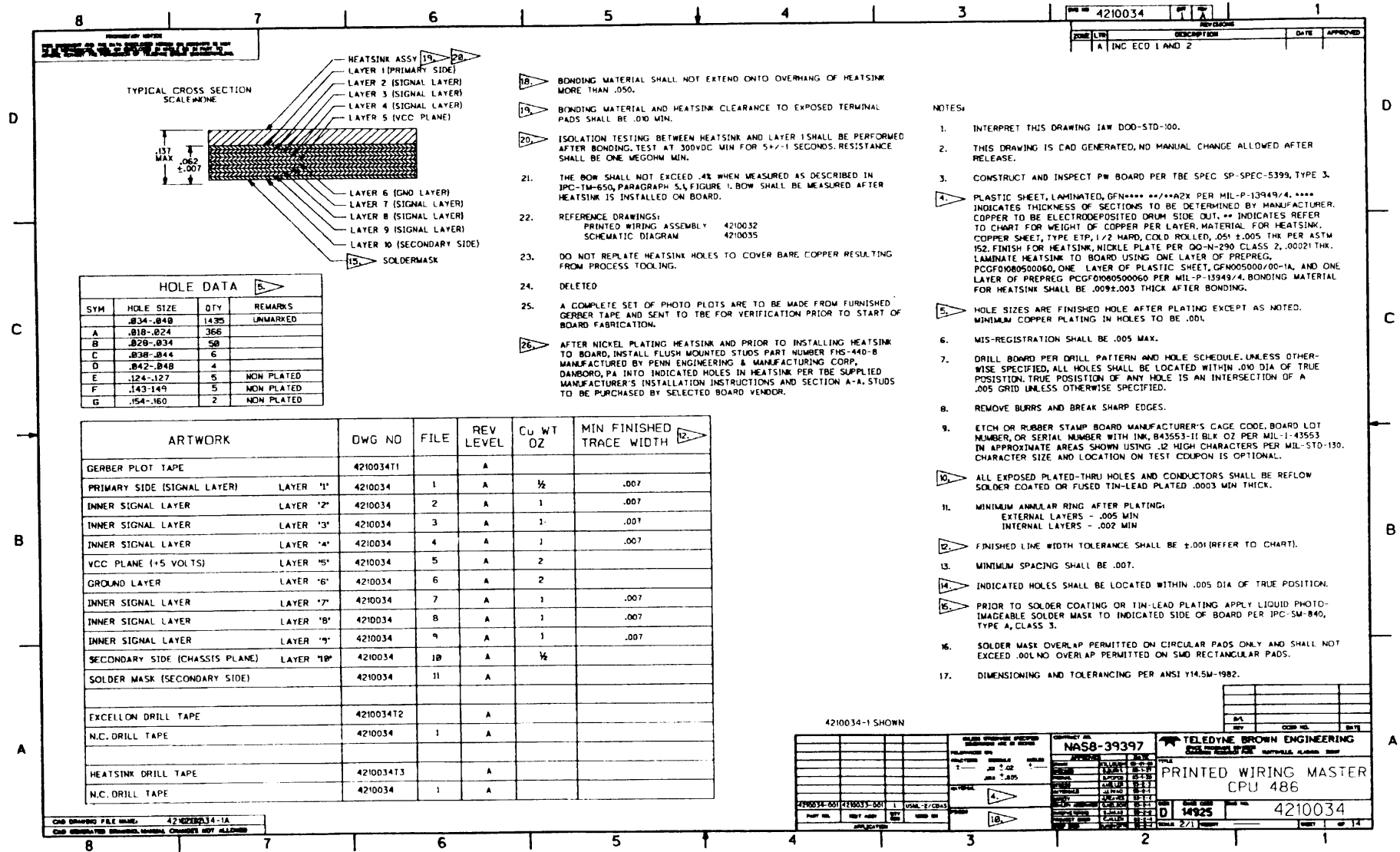
Figure 6-1 Fabrication Drawing
