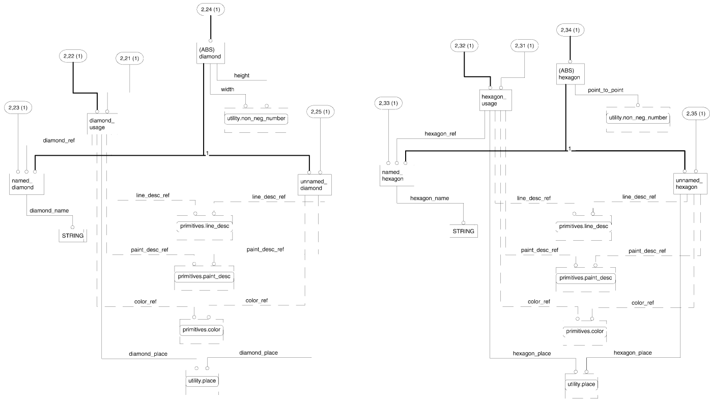
Figure 5-7 EXPRESS-G for Diamond/Hexagon Usage
