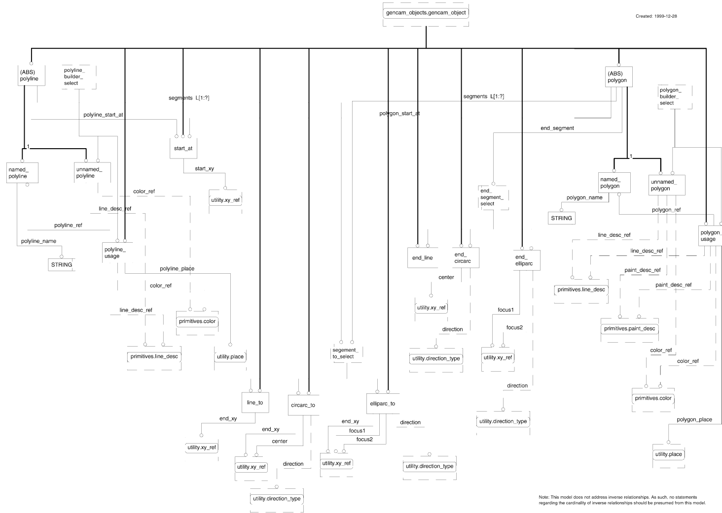
Figure 5-10 EXPRESS-G for Poly Descriptions
