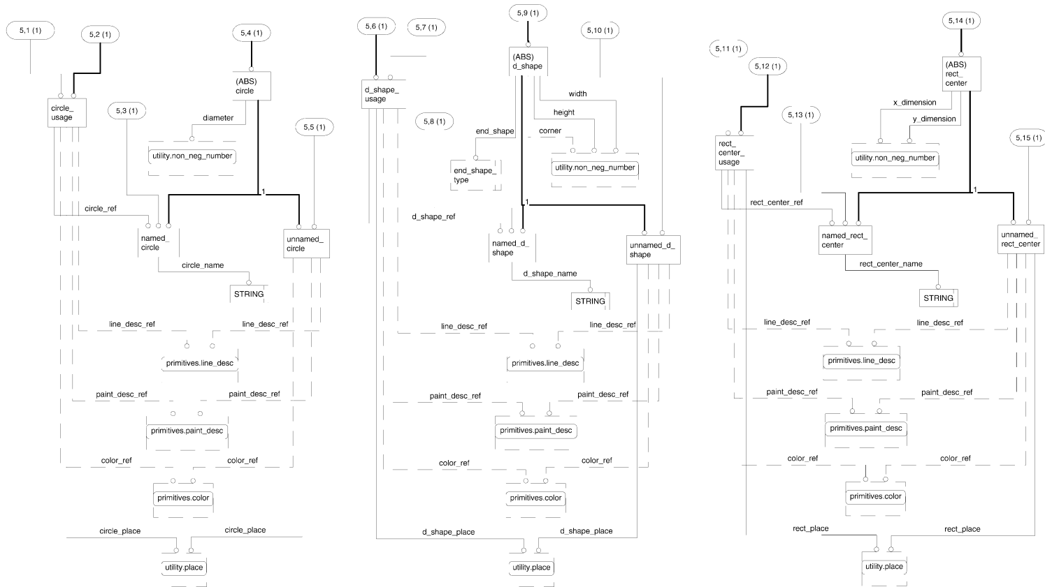
Figure 5-5 EXPRESS-G for Basic PRIMITIVES
