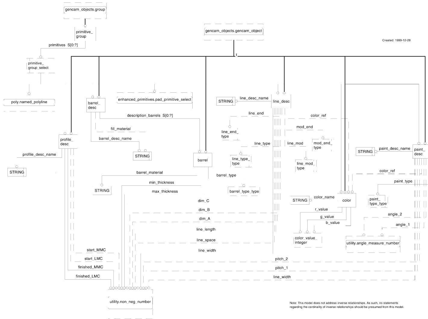
Figure 5-11 EXPRESS-G for Primitive Enhancements
